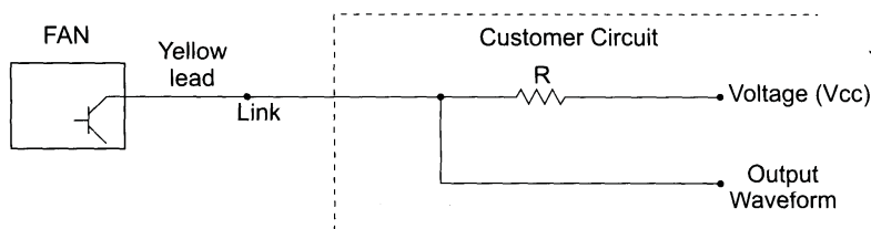
Output Waveform
