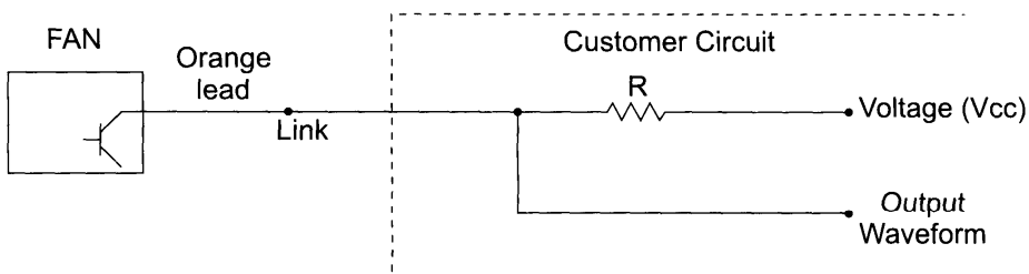
Output Waveform
