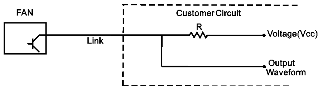
Output Waveform
