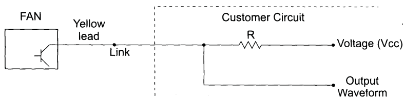
Output Waveform
