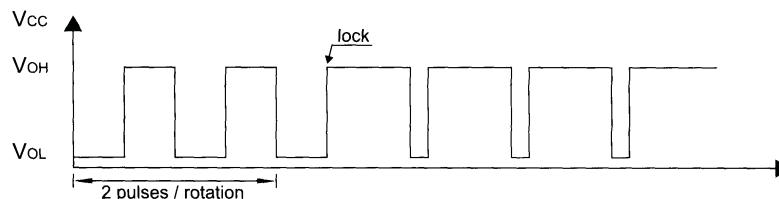
Output Waveform
