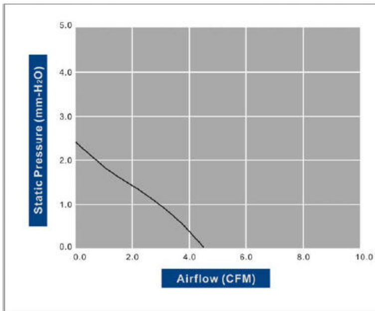
F. Air Flow Performance Curve
