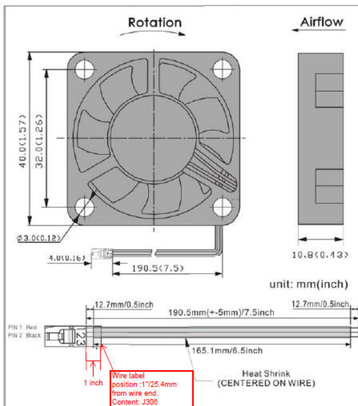
G. Model Drawing
