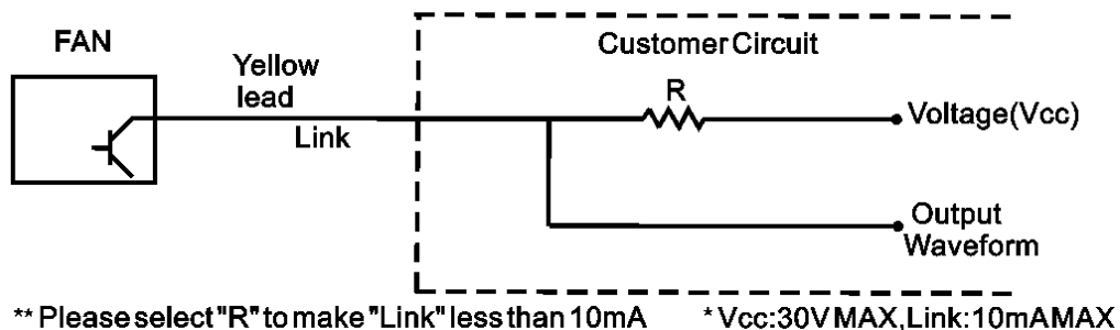
Output Waveform
