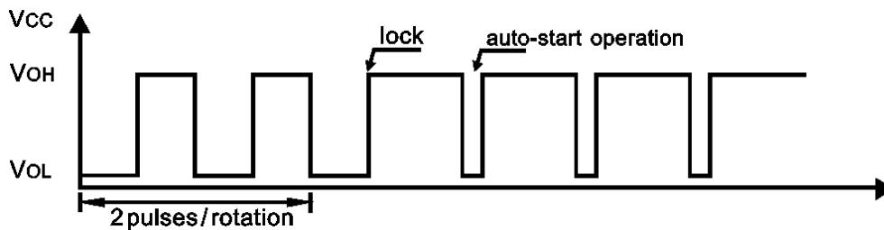
Output Waveform
