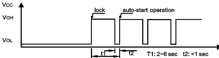
Output Waveform
