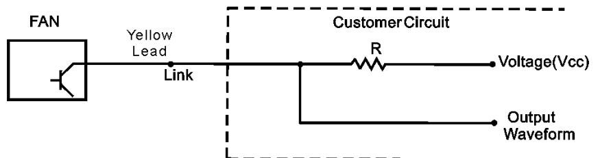
Output Waveform
